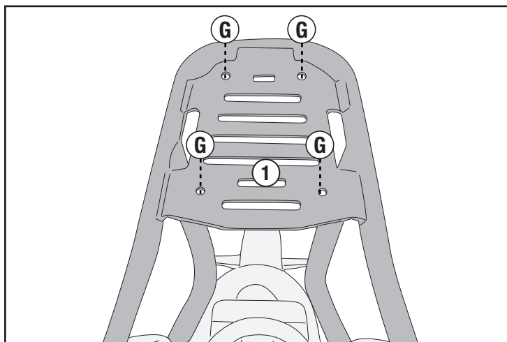
UNIVERSAL MONOLOCK PLATE (SPARE PART Z113C2)
